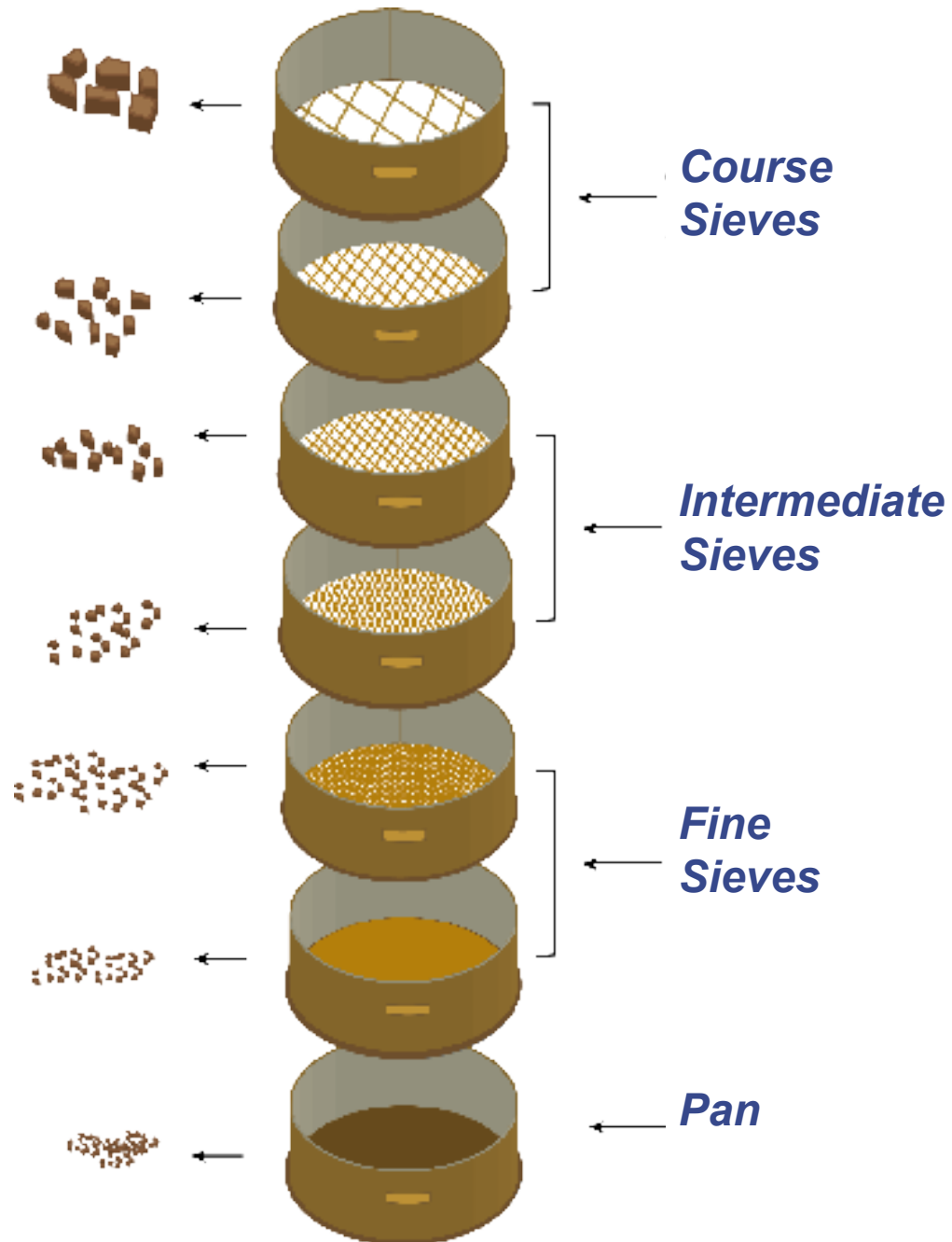
FIGURE 13: Testing gradation.
